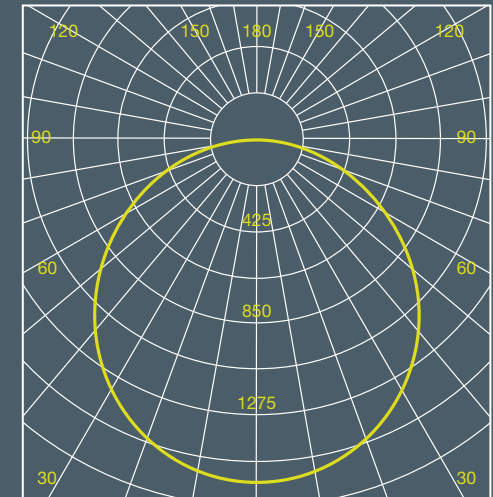
Photometrics diagram shows an even flow of light and enhanced efficacy.
